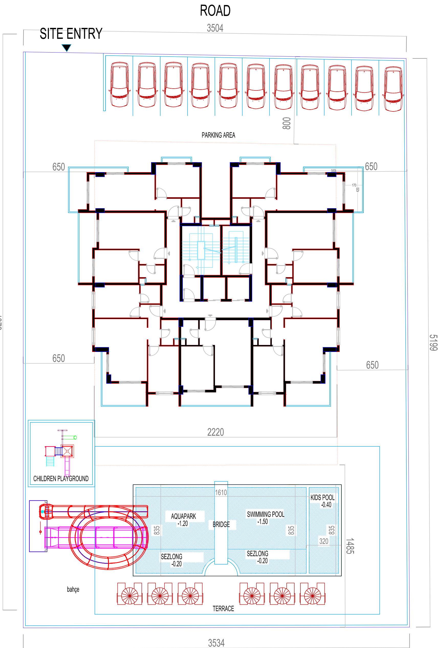
SITE PLAN
